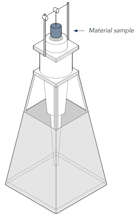
Non-combustibility tester
